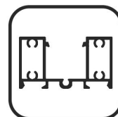
HFVR-H-45 25 X 45 Fix Heavy Vertical
