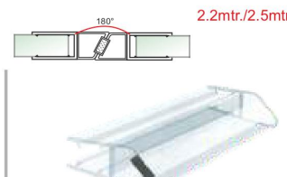
HPS-M-180 Magnetic Seals 180°
