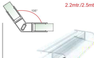
HPS-M-135 Magnetic Seals 135°
