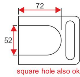
HTLC-SL-11 Sliding Lock with Knob
