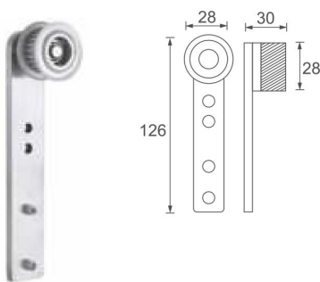
HSL-TFG-02 Long synchronous wheel
