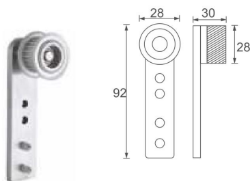
HSL-TFG-03 Short wheel
