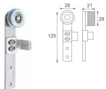
HSL-TFG-04 Long wheel
