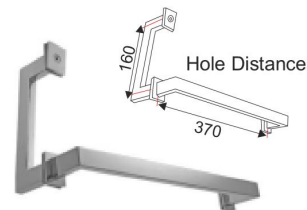
HGH-TB-22 RT Towel Bar Handle Rectangular
