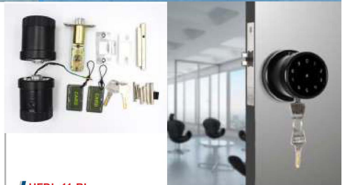
HFDL-11-BL Finger Print & Digital Door Locks
